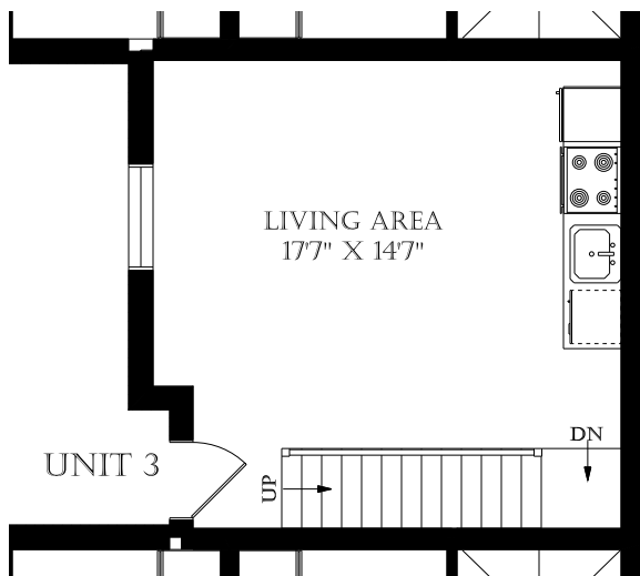
1ST LEVEL 347 SQUARE FEET
