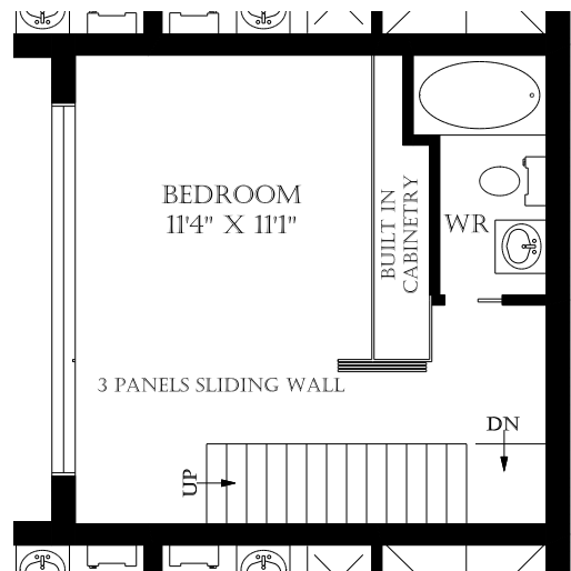
2ND LEVEL 357 SQUARE FEET
